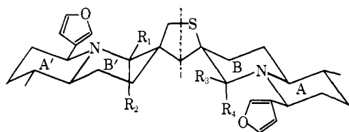
3, R_1 = R_2 = R_3 = R_4 = H
